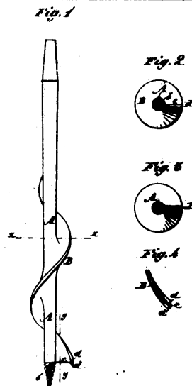
22602 Dimitt's Auger Bit.
