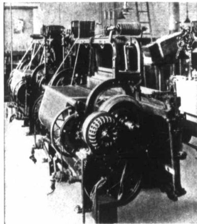
Type CCL Motors Geared to Looms
