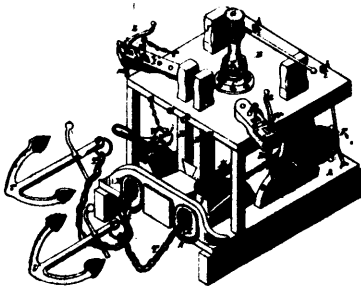
5095 Ste. Marie's Screw-windlass for Steamers and Sailing Vessels.
