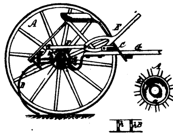
5099 Sharp's Horse-rake.
