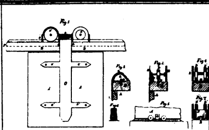
5090 Johnson's Barn Door Hanger.
