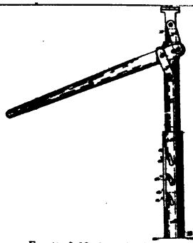
5102 Fayette & Meeker's Lifting Jack.
