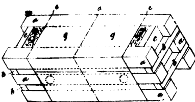
5101 Clay & Sawtell's Fire-lighter.
