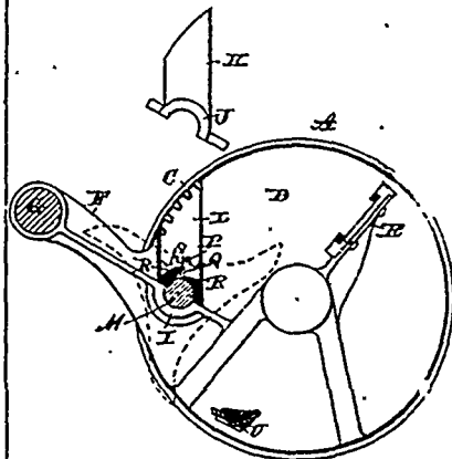
29651 Rogers' Lawn Mower.
