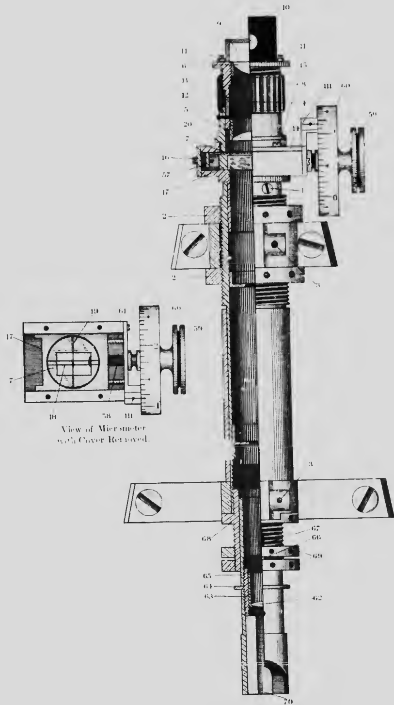
FIGURE 8. Side View and Part Section of Micrometer Microscope.
