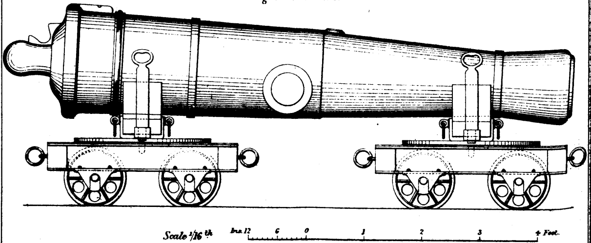
Fig. 16. Elevation.
