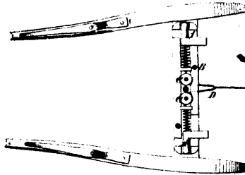
5438 Glover's Horse Detaching Apparatus.
