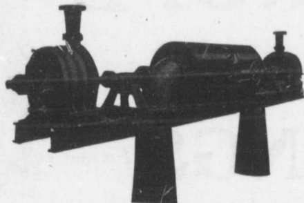
Two Worthington 3-Stage Turbine and McCormack Water Wheels, built for Port Arthur, Ont., Water Works, 1440 gal. per minute against 250 ft. head.
