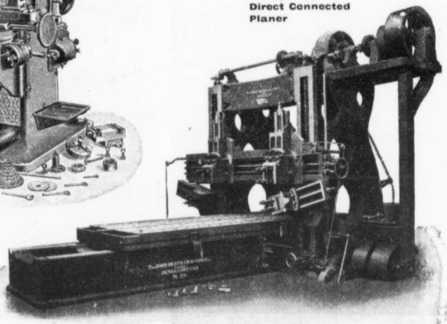
John Bertram & Sons Co. Heavy Duty Direct Connected Planer
