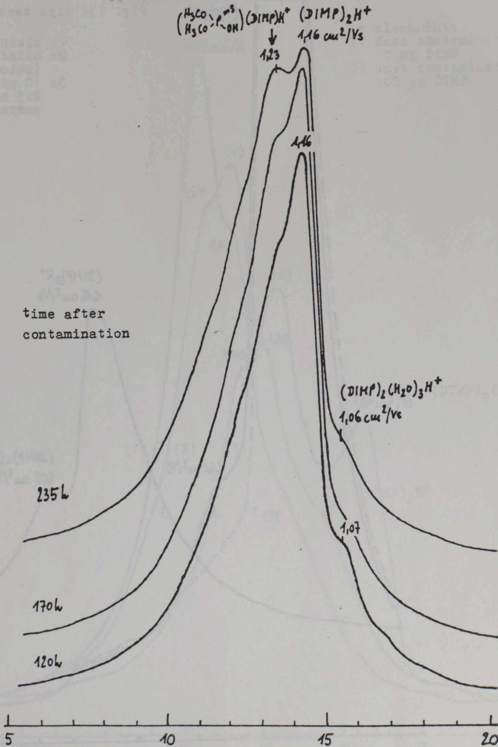
Fig. 12: IMS spectra recorded from packing material (PTFE) which was submerged into a parathion-methyl - DIMP mixture (1 o / 00 ) for 16 hours, time dependence
