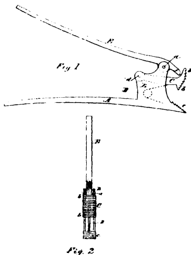
34868 Misener's Horse Shoe Clincher.
