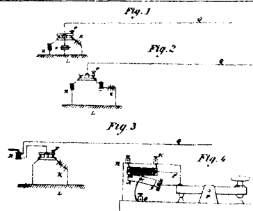
15333 Ryselberghe's Improvements in the Method of, and Apparatus for Preventing Induction in Telegraphic and Telephonic Systems.
