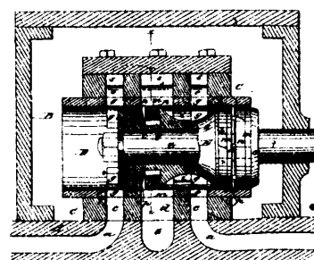
15342 Phelps's Improvements in Steam Valves.
