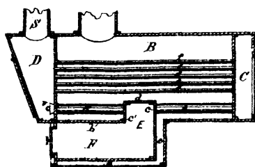
15344 Fitzgibbon's Improvements on Steam Boilers.
