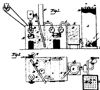
15343 Castner's Apparatus and Process for the Manufacture of Bone Black and Ammonia.
