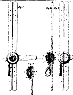
15331 Sloat's Improvements on Rosettes for Bridles.
