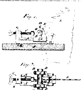
15334 Parson's Improvements on Machines for Jointing and Sharpening Circular Saws.
