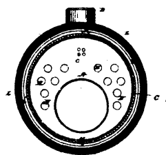
16153 Huber's Improvements on Water Jacket Smoke Boxes.
