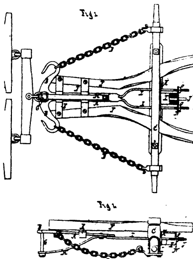
Sebastian's Improvements in Draft Equalizers.
