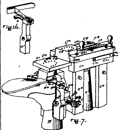
16162 Henderson's Improvements on Heel Nailing Machines.
