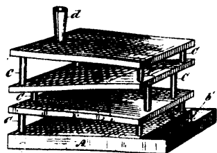
15476 Gayhart's Improvements on Fruit Dryers.
