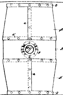
15477 Cutbirtson's Improvement on Metallic Coal Oil Barrels.
