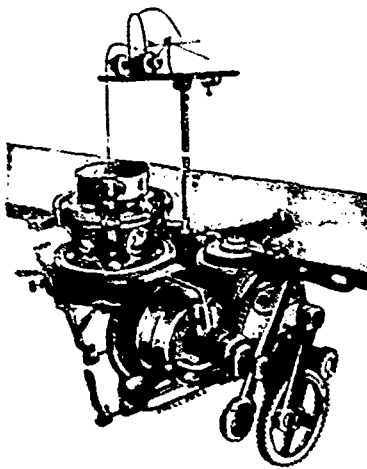
Branson H Automatic Knitting Machine. WINDERS and BOBBINS.
