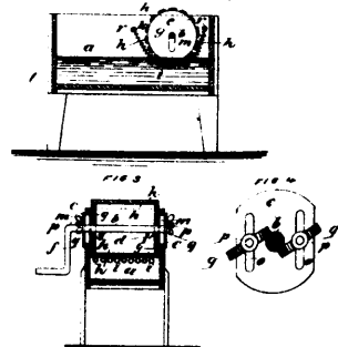
8840 Wilkins &amp; Sawyer's Improvements on Washing Machines.
