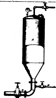
8835 Gaff's Process of Reducing Vegetable Substances to Prepare the same for Saccharification.
