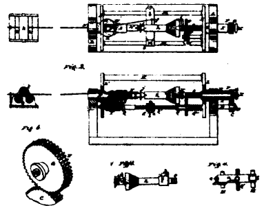
5288 Mattison & Shaw's Spinning Machine.
