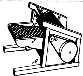
3912 Leadbeter's Grain Separator.
