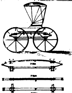
3913 Grimshaw's Carriage and Waggon Spring.
