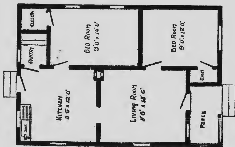
FLOOR PLAN
