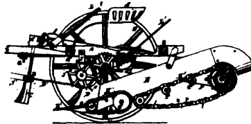
7285 Hopper's Improvements on Potato-diggers.
