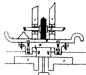
7306 Hennessey's Machine for Cutting the Notches on the Beam of Weighing Scales.
