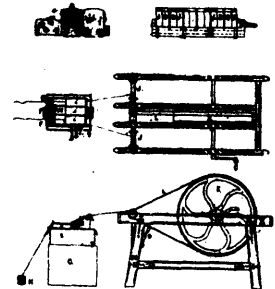
7300 Blakiston's Improvements on Twine Waxing Machines.
