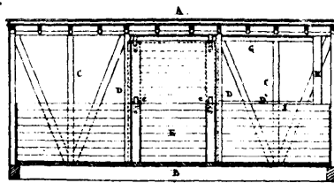
5695 Brydon's Railroad Grain Car Door.
