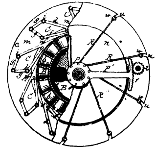
5693 Tait's Water Wheel.
