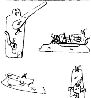
5694 Fenerty's Improvements in Skate Fastenings.
