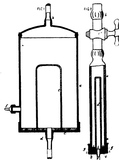
20067 Chamberland's Filter.
