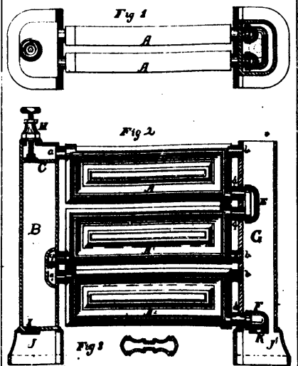
17996 Daniels' Radiator.
