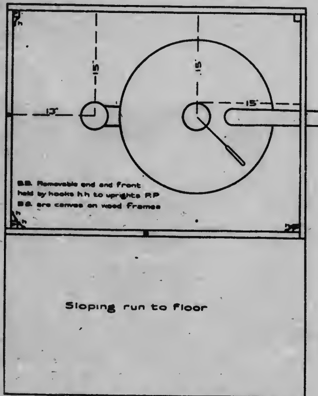
Fig. 4. Showing the floor-plan and arrangement of the hover.
