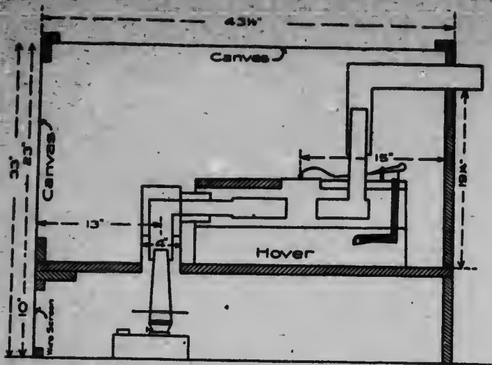
Fig. 3. Showing a section through the middle of the brooder.
