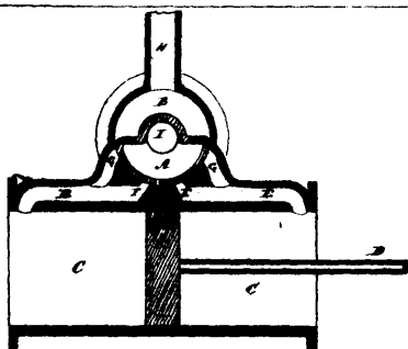
6107 Fairburn's Improvements on Oscillating Valves.
