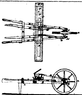
6113 Milne's Improvements on Seeding Machines.
