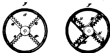
6105 Aubut's Improvements on Root-cutters.
