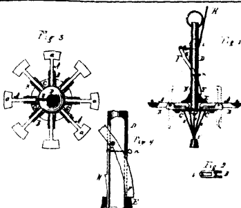
6116 Moore's Apparatus for Walling Wells.
