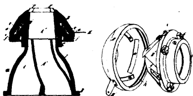
6112 Dunbar &amp; Foss' Improvements on Steam Engine Exhausts.
