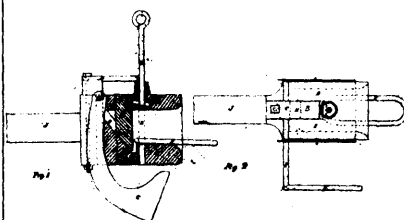
6110 Green's Railroad Car-coupling.
