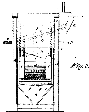
32131 Craig's Sieve Scalper.
