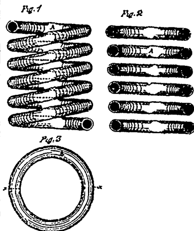
23901 Goewey's Helical Springs.
