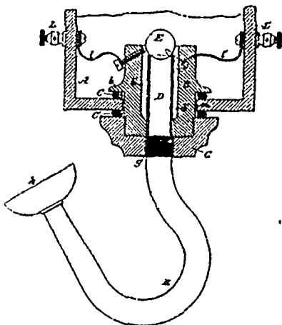
23597 Thomson's Electric Telephone Transmitter.
