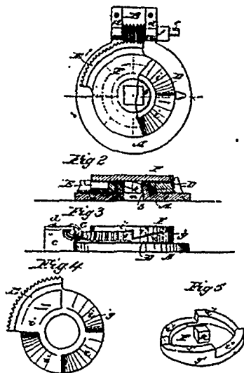
23599 Hornbostel's Billiard Table Leveler.
