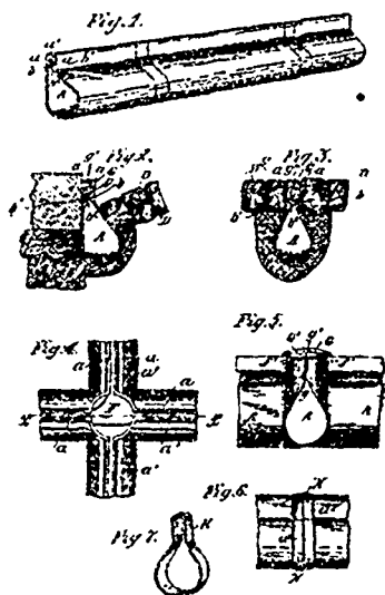
23902 Munroe's Conduit for Electric Wires.
