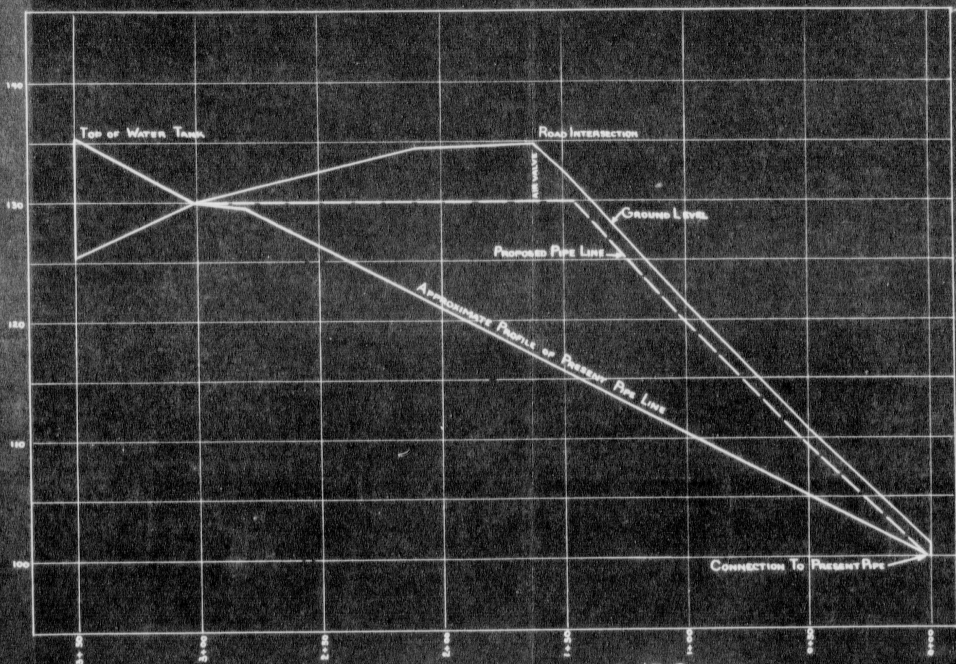
PROFILE OF PROPOSED RELOCATION OF PIPE LINE AROUND LOT D & E. PLAN 2891. SCALE - HORIZ. 1" = 40' VERTICAL 1" = 8'
