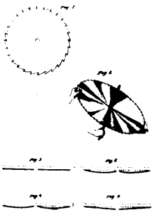
9858 Simonds &amp; Marshall's Improvements in Circular Saws.
