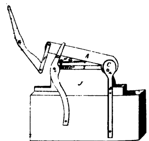
9867 Cook's Machine for Cutting Metal.
