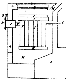
9864 Moore's Improvements on Gas Retorts.
