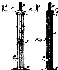
9869 Gullford &amp; Donnelly's Improvements on Railway Jacks.
