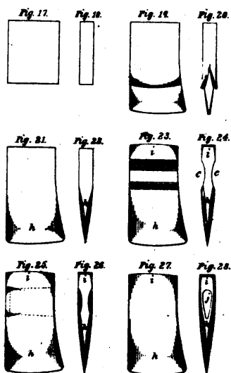
22676 Hammond's Manufacture of Axes.
