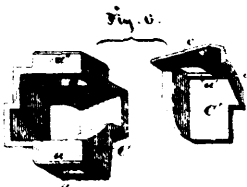
26912 Callander's Harrow.
