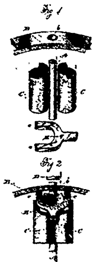
26058 Little's Method of Manufacturing Metal Wheels.
