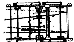
3252 Davis' Improvements on Upright Planofortes.
