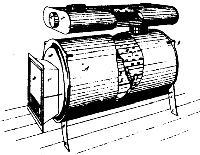
3244 Smith's Improvements on Hot Air Furnaces.
