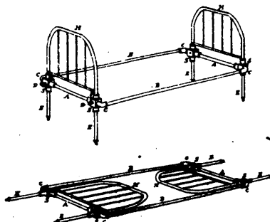
3254 Hobb's Folding Pipe Bedstead.
