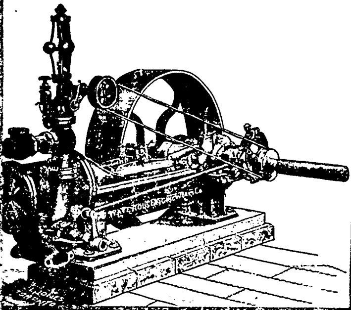
is Style made in 12, 16, 20, 25 and 30 Horse Power.
