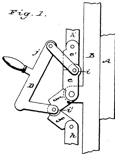
27530 Isbell's Mechanical Movement.
