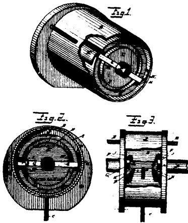
27527 Hills' Steam Engine.
