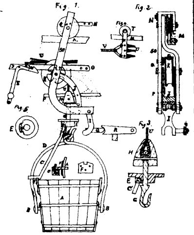
27526 Ryan's Apparatus for Hoisting and Moving Earth.
