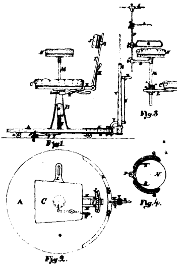
27531 EnDean's Photographer's Chair.
