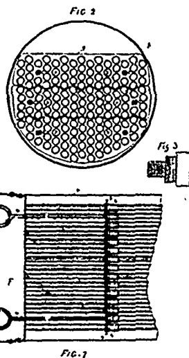
24507 Smith &amp; Melcklejohn's Roller Cleaner.
