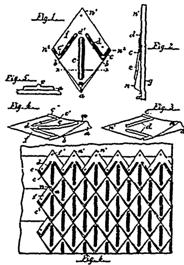
24513 Lemler's Metallic Roofing Tile.
