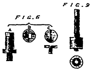
HOW TO MAKE AN ECCENTRIC CHUCK.
