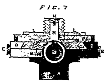
HOW TO MAKE AN ECCENTRIC CHUCK.
