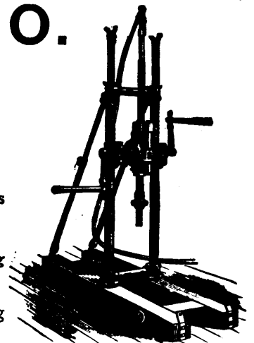
"Bravo" Hand Power Drill. Capacity. 400 feet. 1 3/4", hole 12-16"
