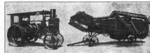
Case 20-40 Kerosene Tractor and 32x54 Thresher with All Attachments A Popular Combination that Satisfies Every Owner
