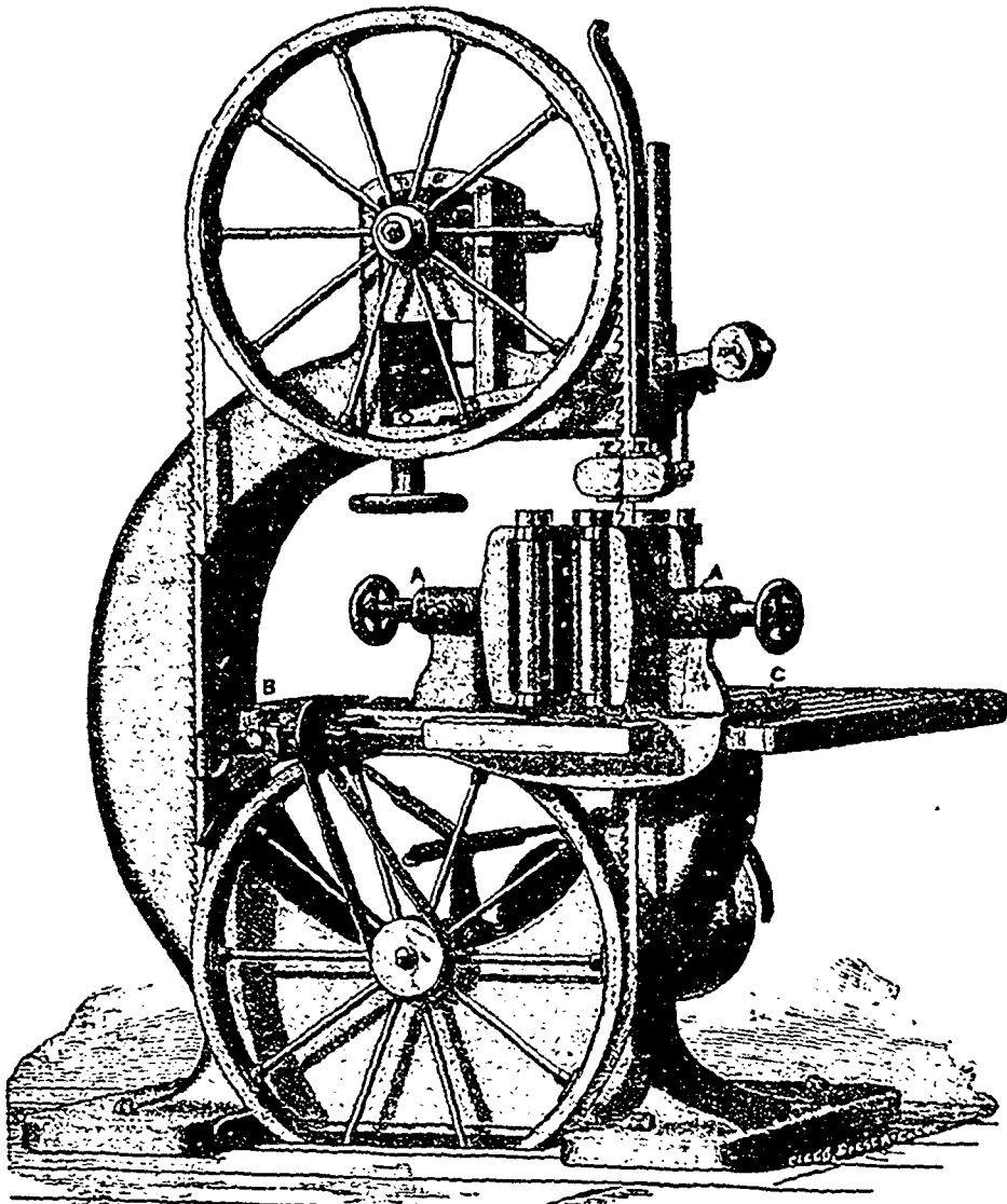
OUR NEW STANDARD BAND RE-SAWING MACHINE.
