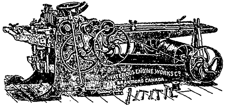
The Champion Planer, Matcher and Moulder. Planes 24 x 3/4 to 6 inch thick. Matches and Sizes 15 inches wide. Has extra 7 in. Slotted Head for Moulding.
