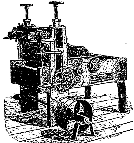
The Little Giant Planer, Matcher and Moulder Combined.
