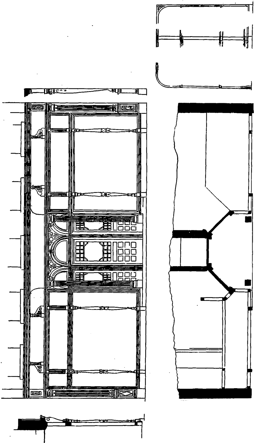
STORE FRONTS FOR JOS. MCCAUSLAND & SON, TORONTO. DARLING & CURRY, ARCHTCTS.
