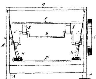
12440 Doherty's Improvements in Thrashing Machines.
