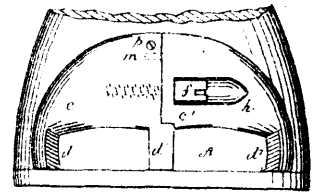
12435 Robarge's Improvement on Toe Weights for Horses..
