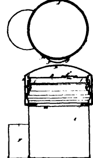
2539 Chinnock's Sheet Metal Can.
