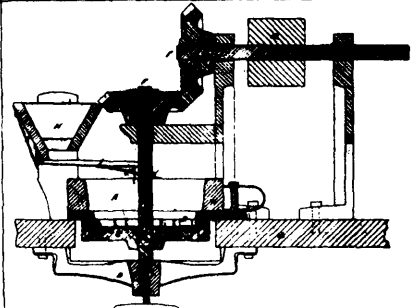
2542 Kaiser's Grain or Corn Crushing Mill.
