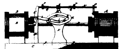
2548 Tesseyman &amp; Howard's Valve Gear for Direct-acting Steam Engines.
