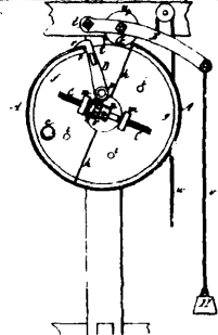
2545 Coapman's Machine for Forming Barrel Hoops.
