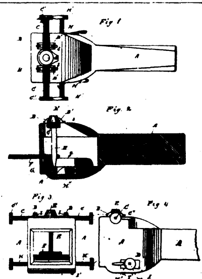
20279 Crowell's Car-Coupler.
