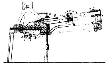
6896 Rittenhouse & Weaver's Improvements on Tack Machine Feeders.
