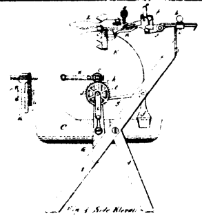
6887 Stevens' Machine for Grinding Harvester Knives.
