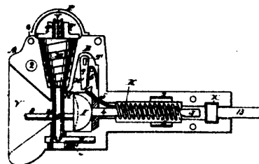
4007 Dolsen's Automatic Car-coupling.
