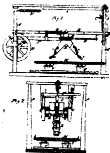
4005 Head's Leather Scouring Machine.
