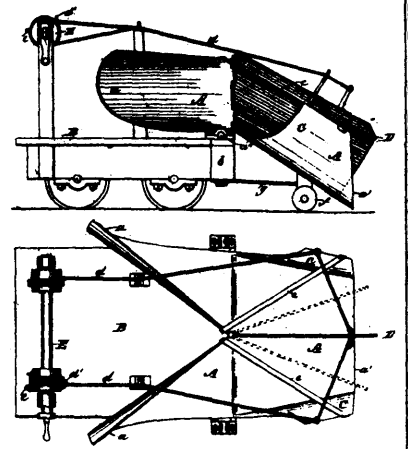
16053 Resley's Improvement on Snow Ploughs.
