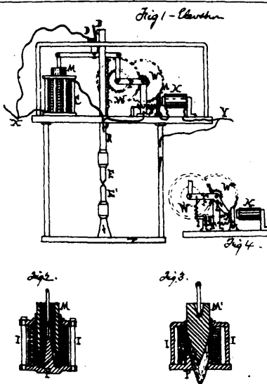
16051 Thomson's Improvements on Electric Air Lamps.
