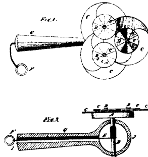
9584 Erwin's Improvements on Chromatrope Toys.
