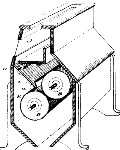
26508 Wilson &amp; Thomson's Oat Meal Chopping Mill.
