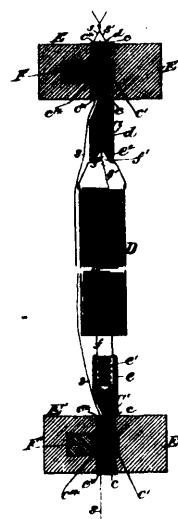
26507 Gilbert's Wire Netting Machine.
