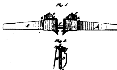
7682 Keen's Improvements on Car-Couplings.
