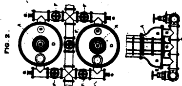
7675 Newton's System for Regulating the Continual Supply of Purified Water and Continual Discharge of Refuse Water.
